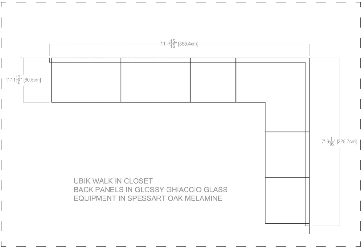
UBIK - PLAN VIEW
